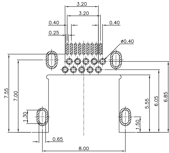
RECOMMENDED PCB LAYOUT(TOP VIEW) (THICKNESS=1.20±0.05mm) (TOLERANCE=±0.05mm)
