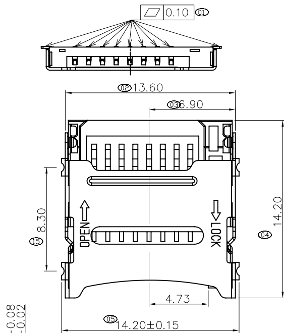
SLIDE SHELL OPEN
