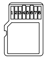
T-FLASH CARD SCALE 2:1
